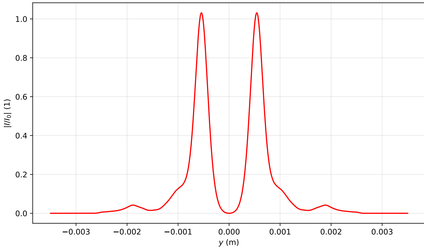
Intensity profile I(x=0, y, z=1.831)/I_0 , P_{in}=7.0P_{cr} , artificial time
